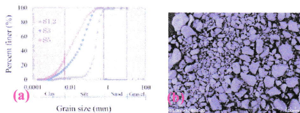
Fig5. (a) grain size distribution of soil samples (b) SEM image of sample S2
